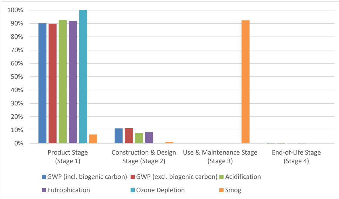
Figure 2. Impact Category Result Breakdown by ISO 21930 Stage. Based on average, mixed Part A + Part B, FIRETEX C69 coating system.
