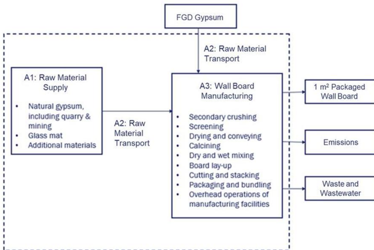
Figure 3-1: Simple flow chart providing details on the Product Stage (A1 to A3) for 5/8" DensElement® Sheathing
