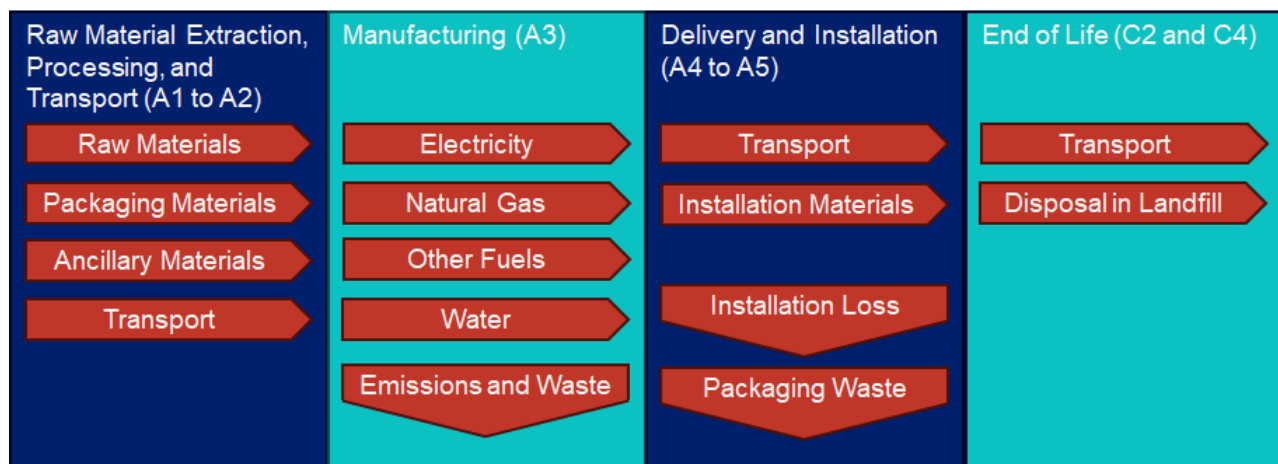
Figure 1-1: Simplified process flow diagram for 5/8" ToughRock® Lite-Weight Fire-Rated Gypsum Board
