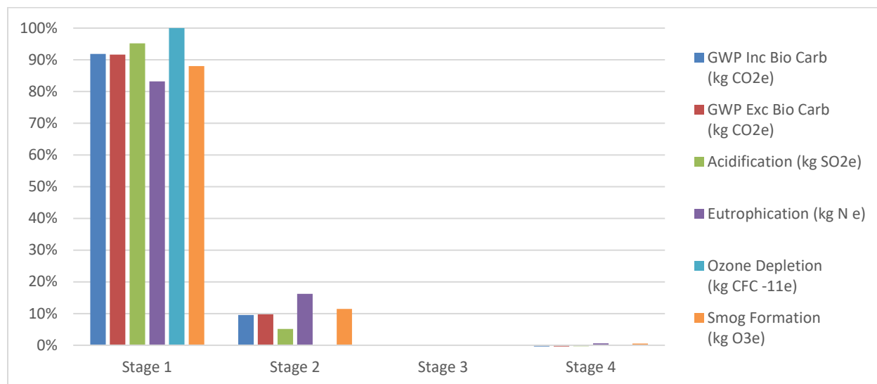
Figure 2. Impact Category Result Breakdown by ISO 21930 Stage for Average Solo® 100% Acrylic Interior/Exterior Formulation.
