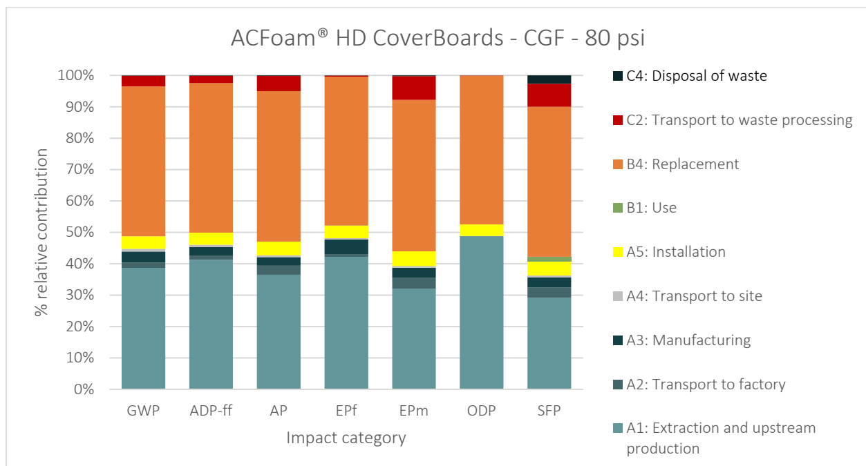
Figure 5: Contribution of life cycle information modules to the potential environmental impacts of 1m 2 of installed ACFoam® HD CoverBoards, CGF, 80 psi, for 75 years.
