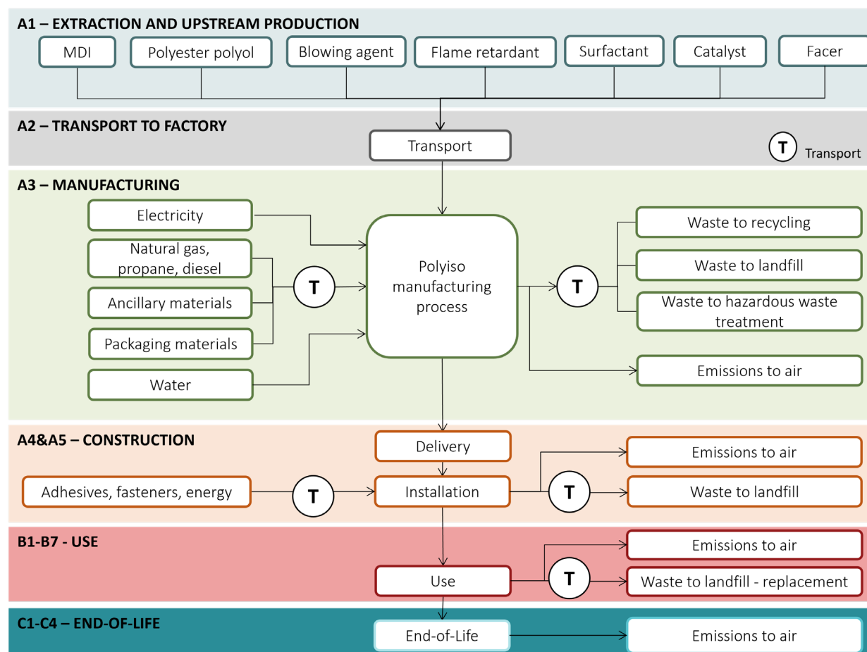
Figure 4: Cradle-to-gate with options system boundaries of polyiso product LCA.
