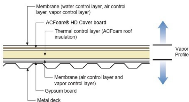
Figure 2: Typical roof assembly with polyiso ACFoam® HD CoverBoard installed between the insulation and the roof membrane.
