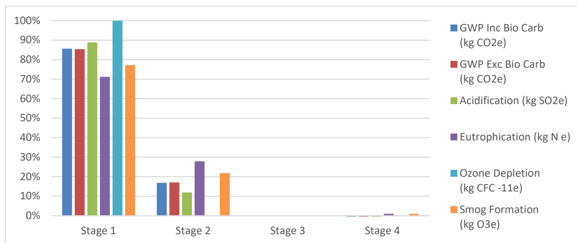
Figure 2. Impact Category Result Breakdown by ISO 21930 Stage for Average PVA Interior Latex Drywall Primer & Sealer Formulation.
