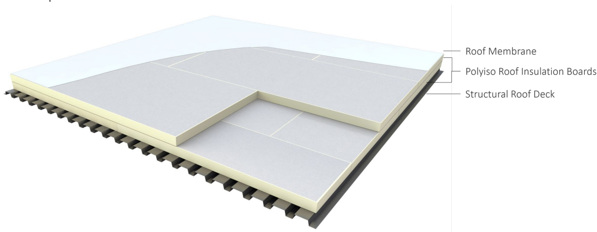
Figure 3: Typical roof assembly with polyiso roof insulation boards installed direct-to-steel deck.
