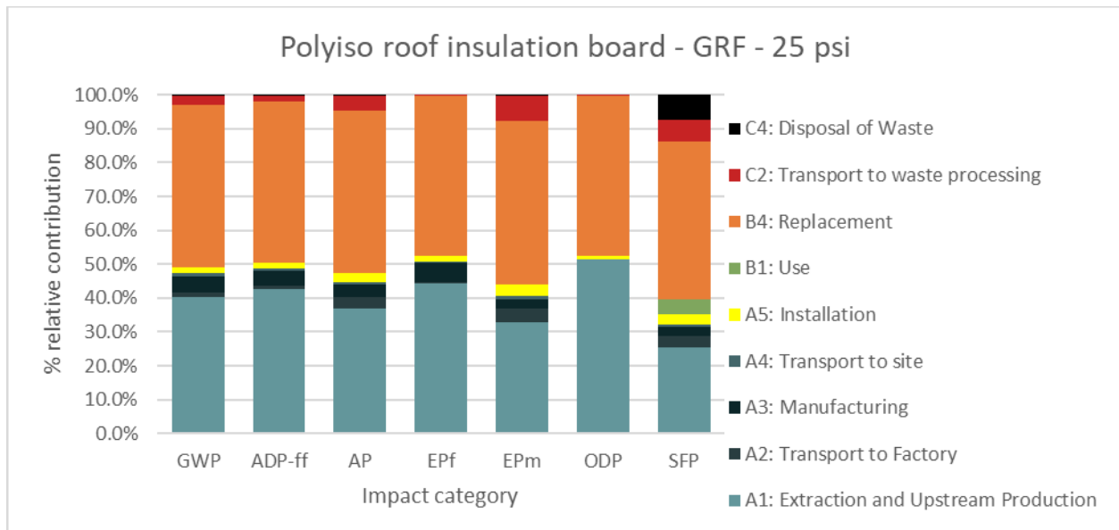
Figure 9: Contribution of life cycle information modules to the potential environmental impacts of 1m 2 of installed polyiso roof insulation board, GRF, 25 psi, for 75 years.
