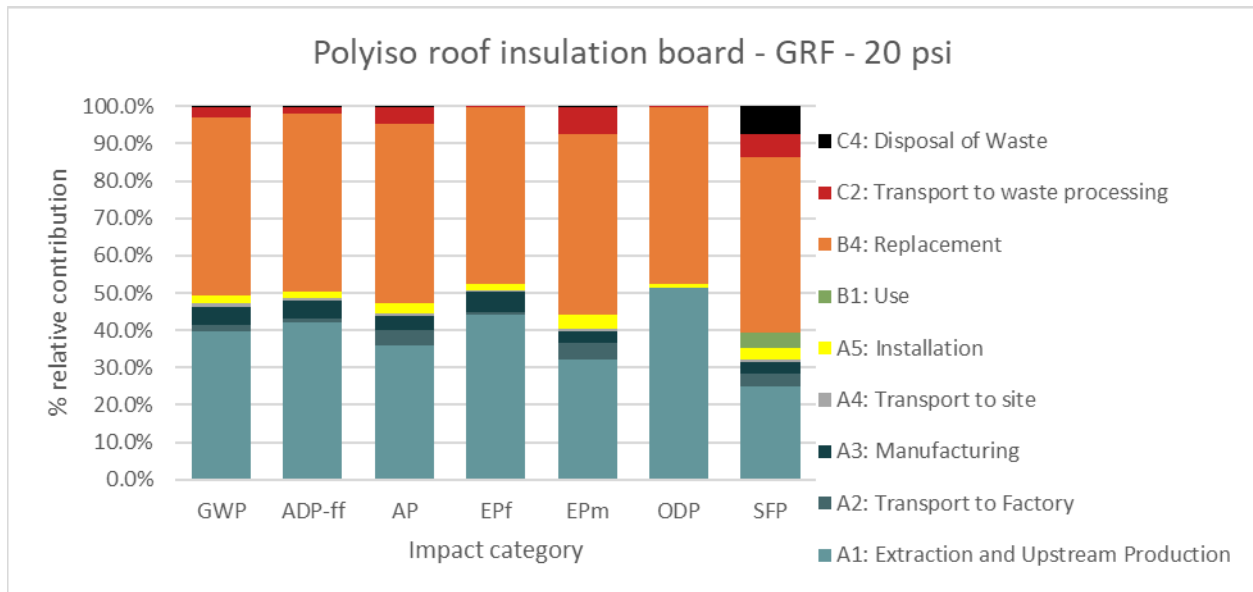
Figure 8: Contribution of life cycle information modules to the potential environmental impacts of 1m 2 of installed polyiso roof insulation board, GRF, 20 psi, for 75 years.
