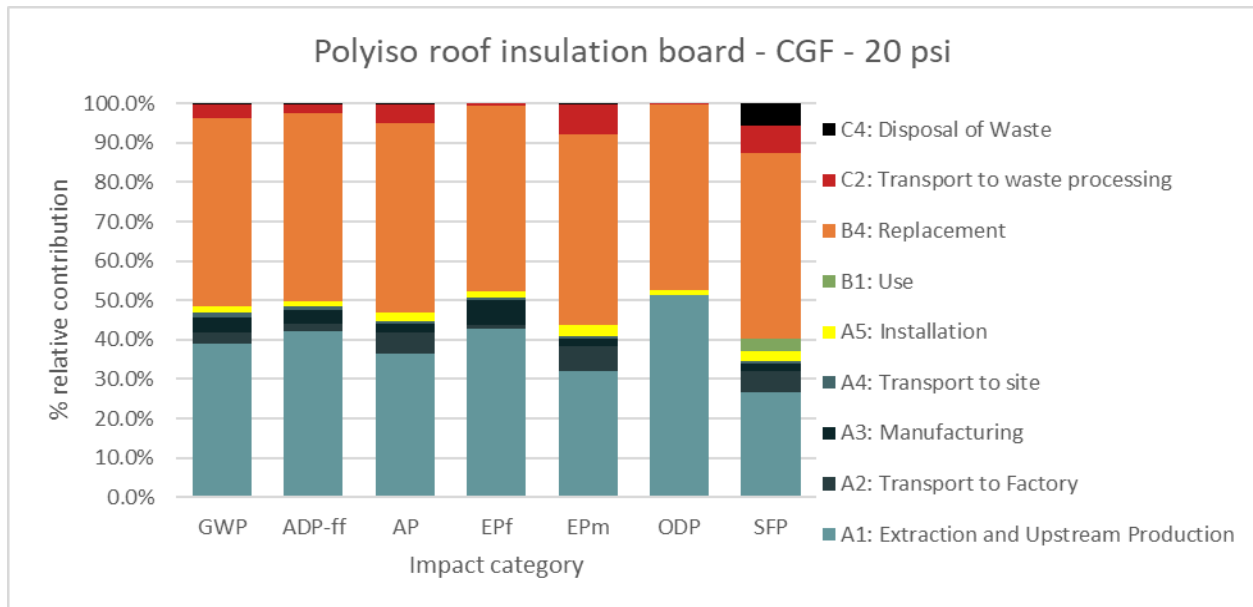
Figure 6: Contribution of life cycle information modules to the potential environmental impacts of 1m 2 of installed polyiso roof insulation board, CGF, 20 psi, for 75 years.
