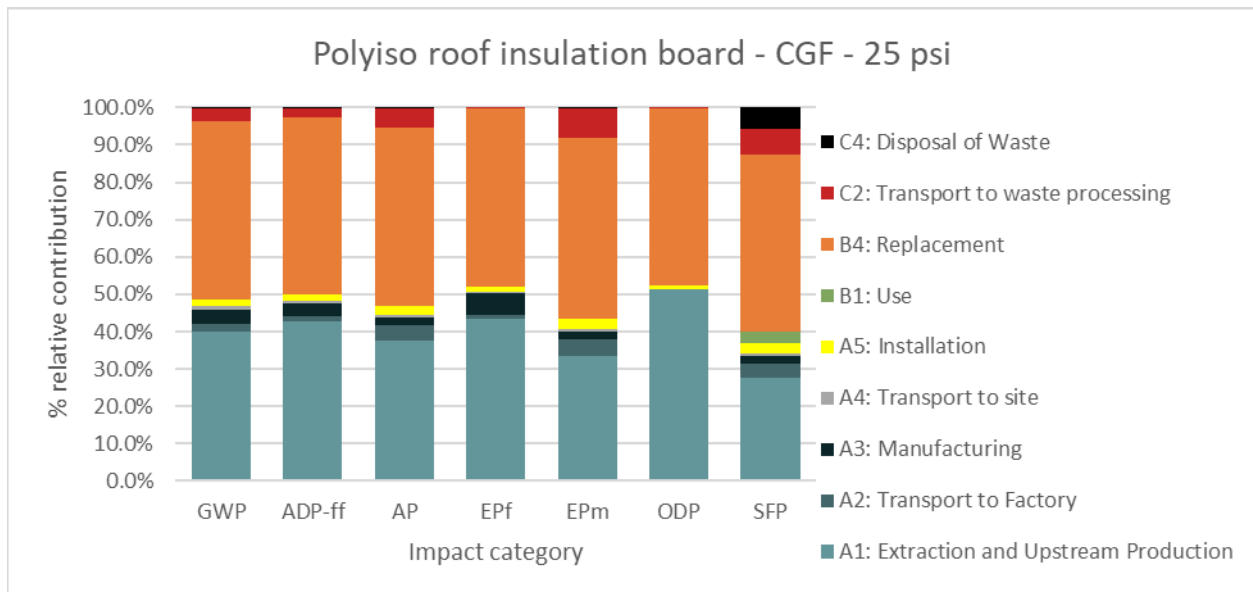
Figure 7: Contribution of life cycle information modules to the potential environmental impacts of 1m 2 of installed polyiso roof insulation board, CGF, 25 psi, for 75 years.
