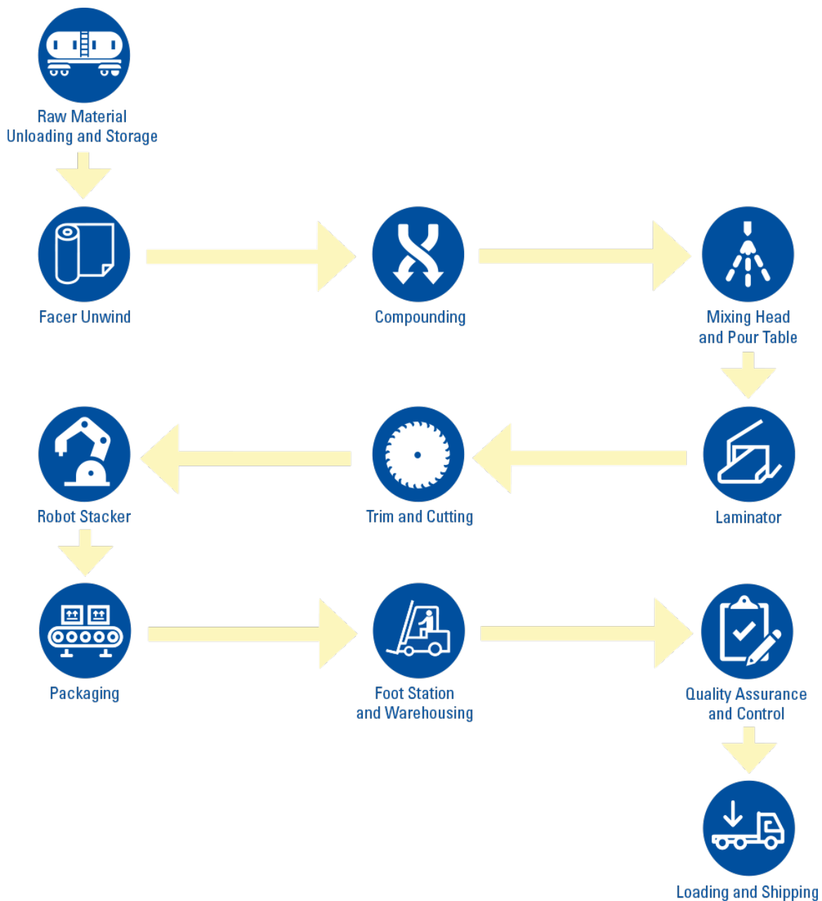
Figure 4: Illustration of the polyiso insulation manufacturing process.
