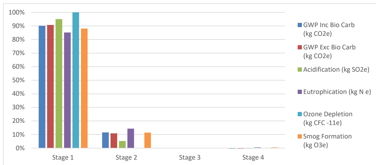
Figure 2. Impact Category Result Breakdown by ISO 21930 Stage for Average Duration® Exterior Acrylic Latex Formulation.
