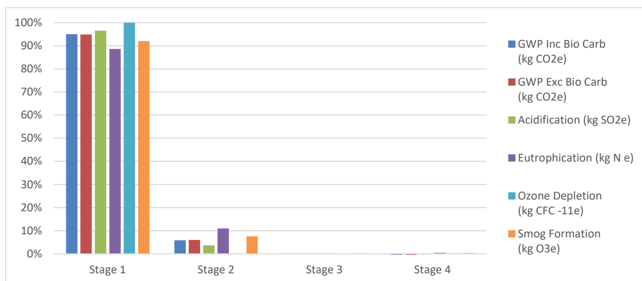
Figure 2. Impact Category Result Breakdown by ISO 21930 Stage for Average Forte™ Urethanized Acrylic Formulation.
